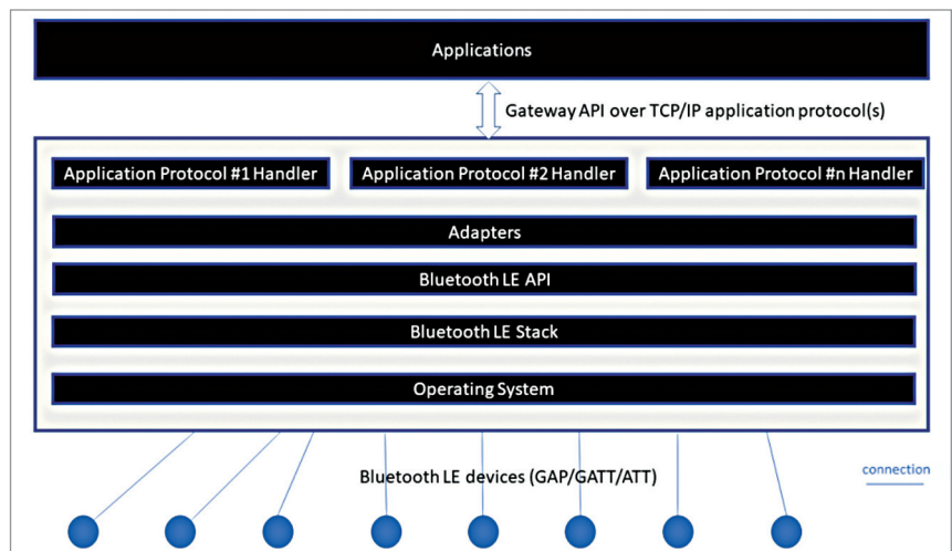
Fig. 5: Gateway logical architecture
